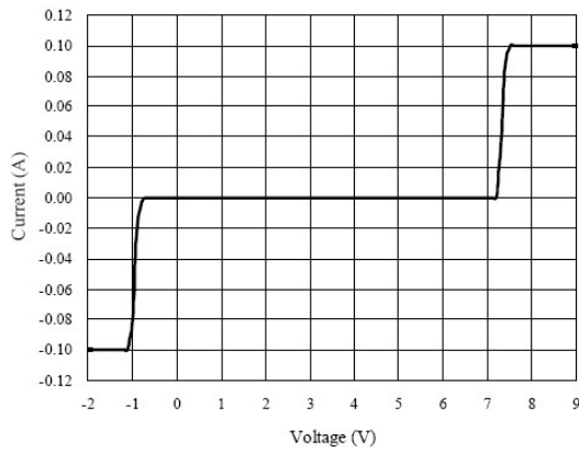
Voltage Sweeping of I/O to GND
