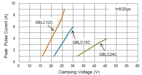
Fig 6 Clamping Voltage vs Peak Pulse Current
