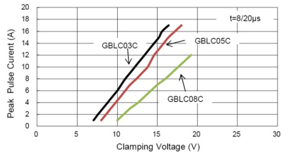
Fig 5 Clamping Voltage vs Peak Pulse Current
