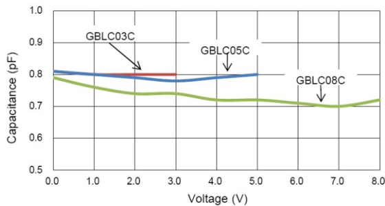
Fig 3 Voltage vs Capacitance
