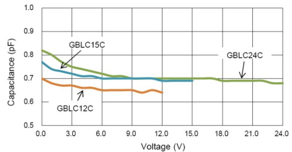
Fig 4 Voltage vs Capacitance
