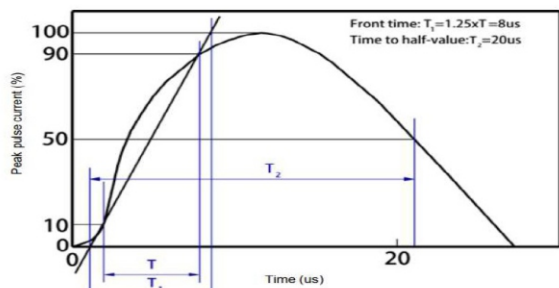
Fig 1 8/20 \mu s Waveform per IEC61000-4-5
