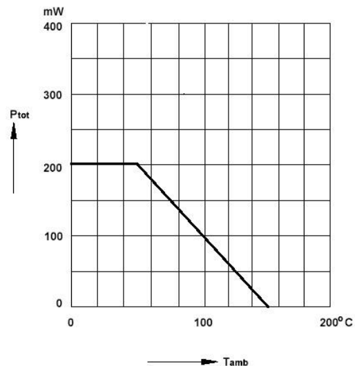
Admissible power dissipation versus ambient temperature
