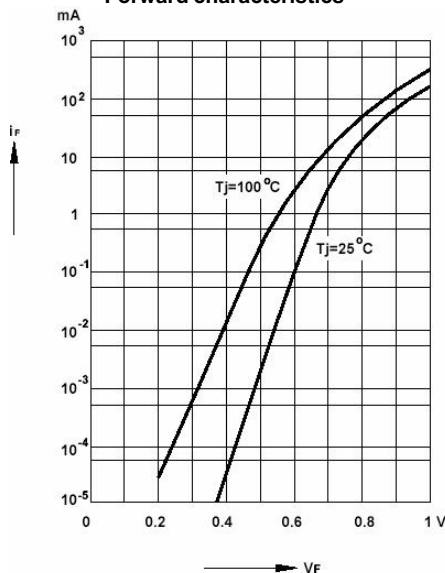
Forward characteristics
